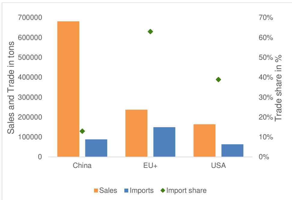
Figure 10. Imports and sales of LIB in three main markets
